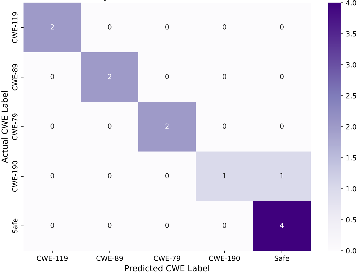
Code Vulnerability Classifier - Confusion Matrix (XGBoost)
